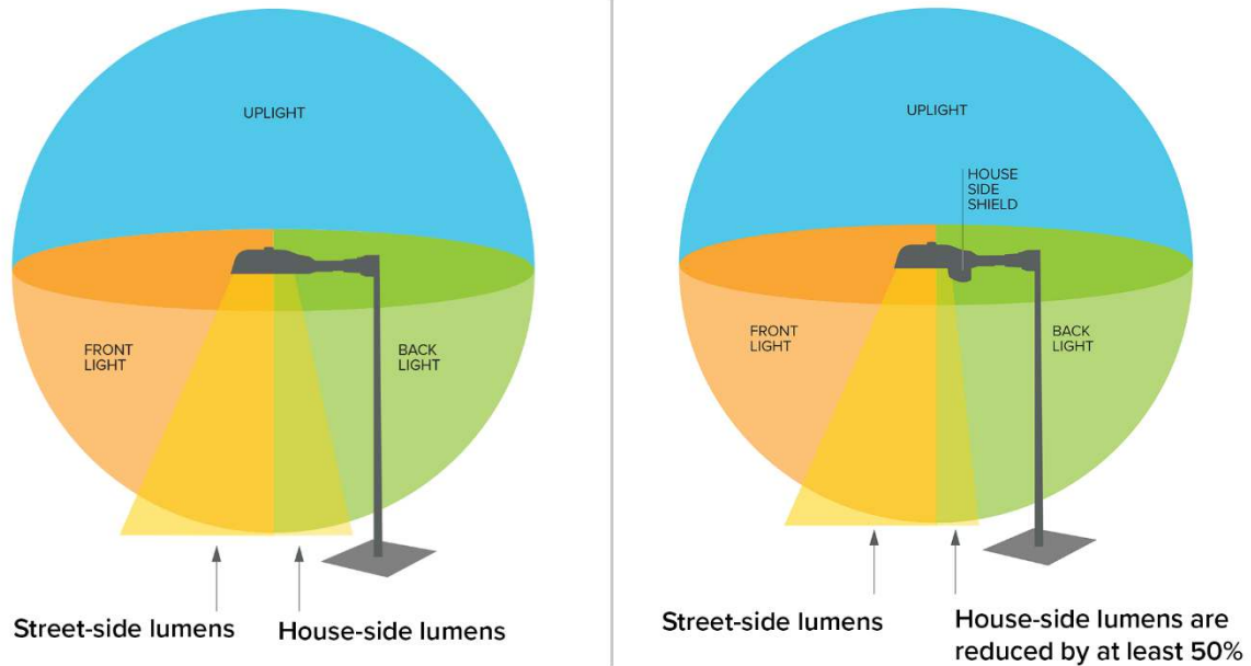
Figure 2: Example of a hypothetical product with a house-side-shield (HSS) (right image) and without (left image). The one with a HSS would be eligible for a shielding efficacy allowance if the house-side lumens were reduced by at least 50% compared to those from an unshielded equivalent product. It is important to note that shielding efficacy allowances for other shield types will require different reductions in house-side or street-side lumens, per Table 26 .
